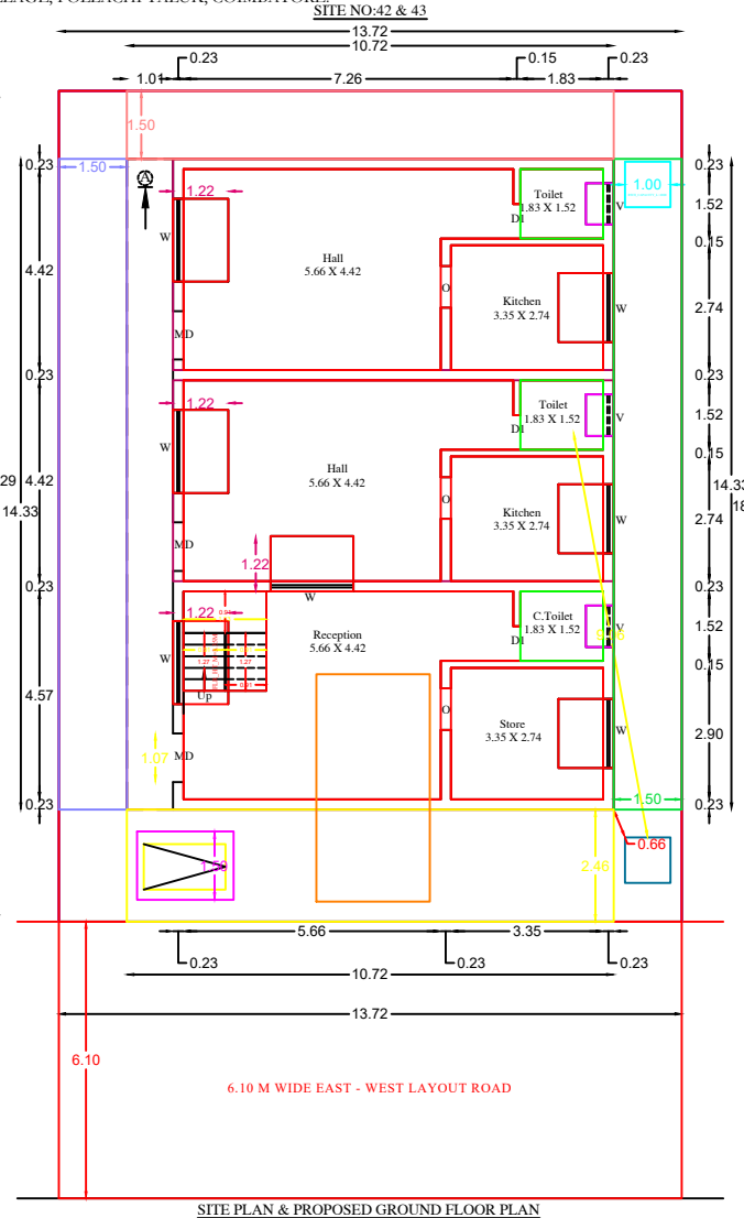
SITE PLAN & PROPOSED GROUND FLOOR PLAN
