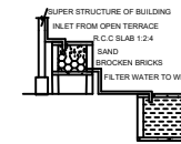
RAINWATER HARVESTING
