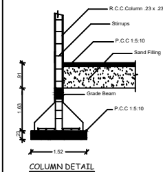
COLUMN DETAIL
