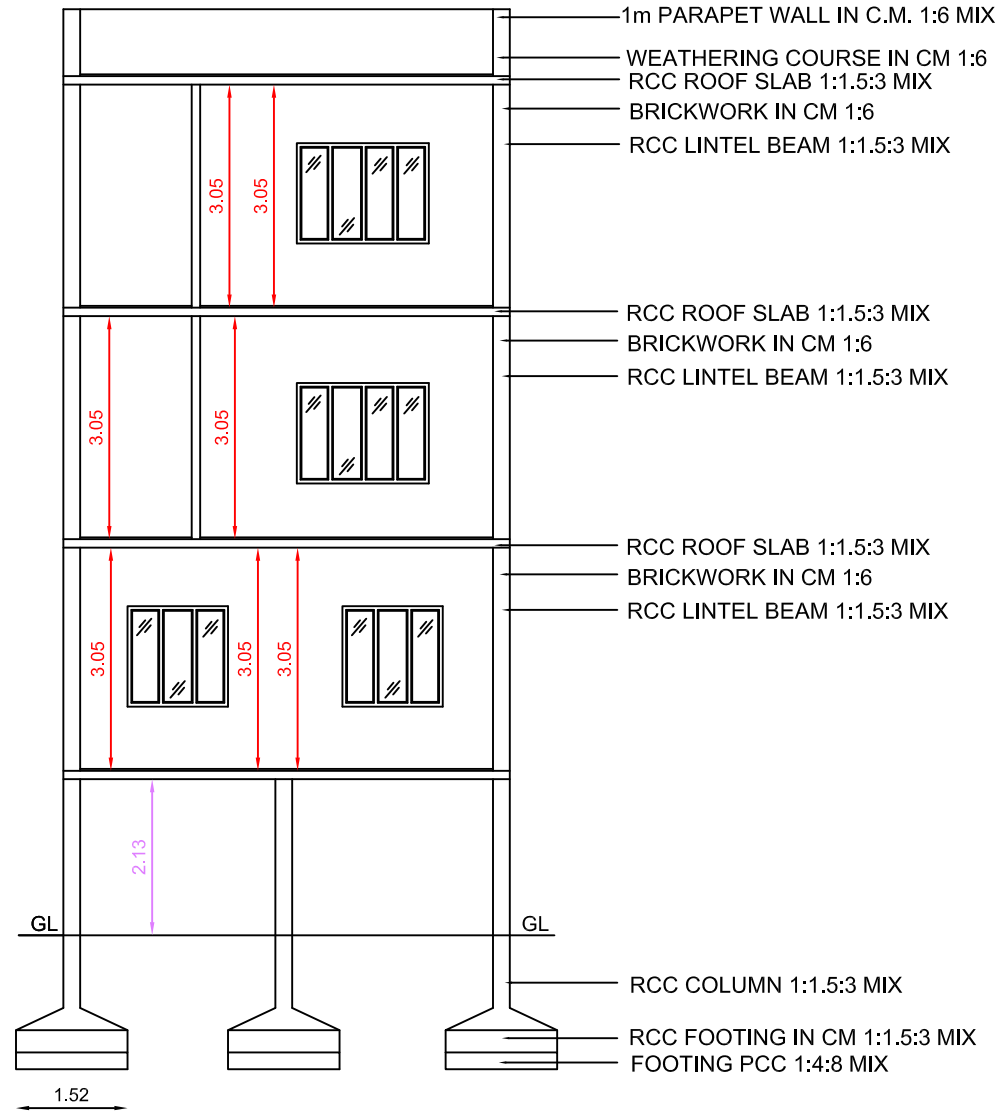
CROSS SECTION ON XY
