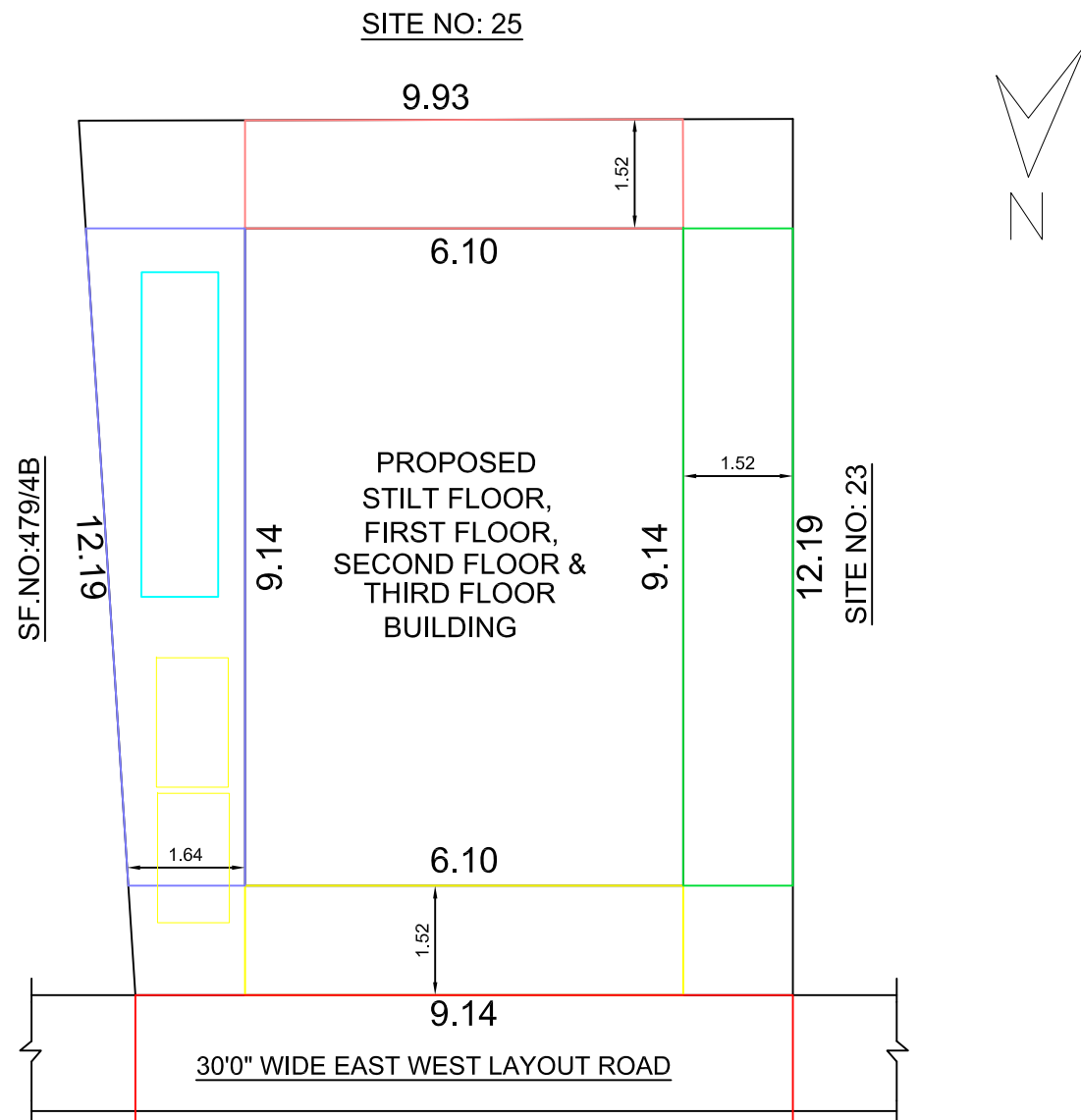
SITE PLAN
