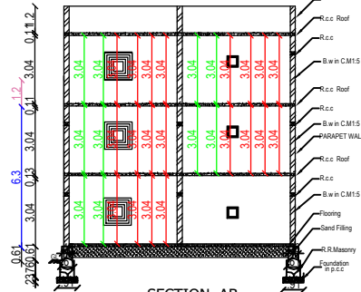
SECTION AB
