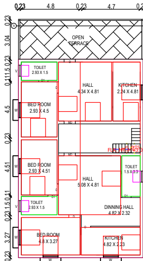
PROPOSED SECOND FLOOR PLAN
