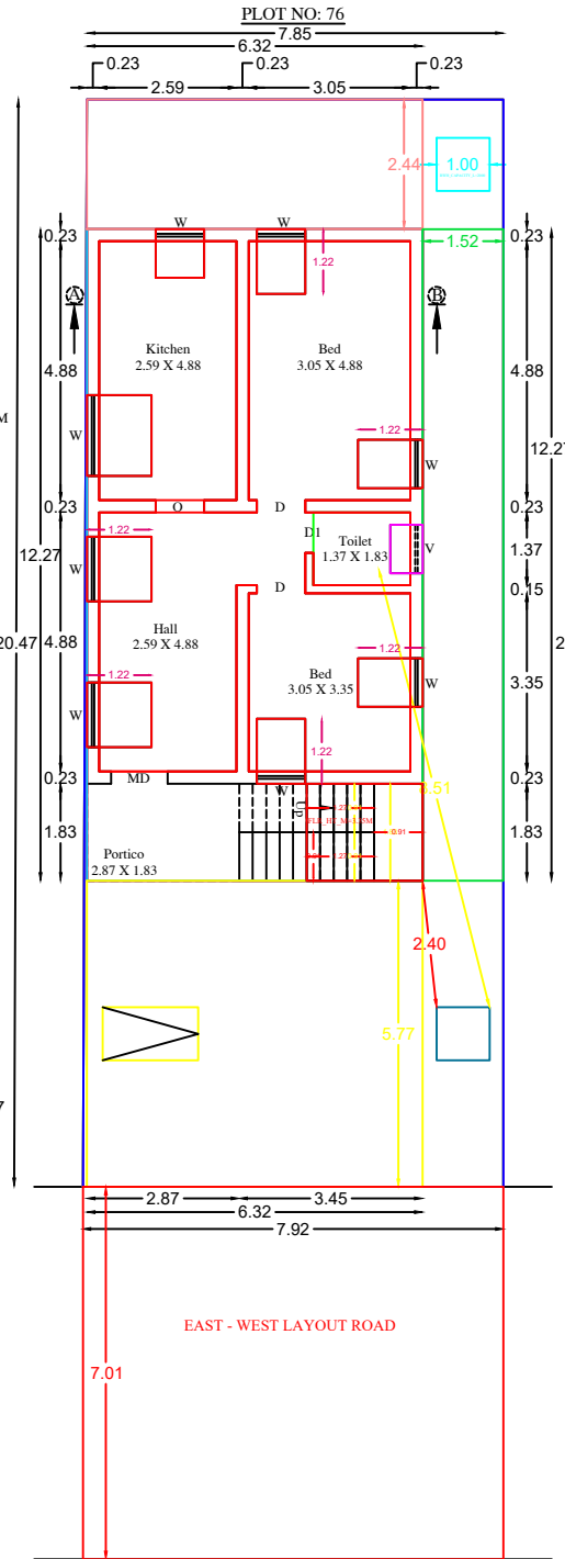
SITE PLAN & EXISTING GROUND FLOOR PLAN
