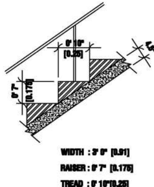
STAIRCASE DETAILS:
