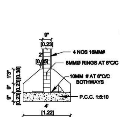
Coulumn Foundation Details
