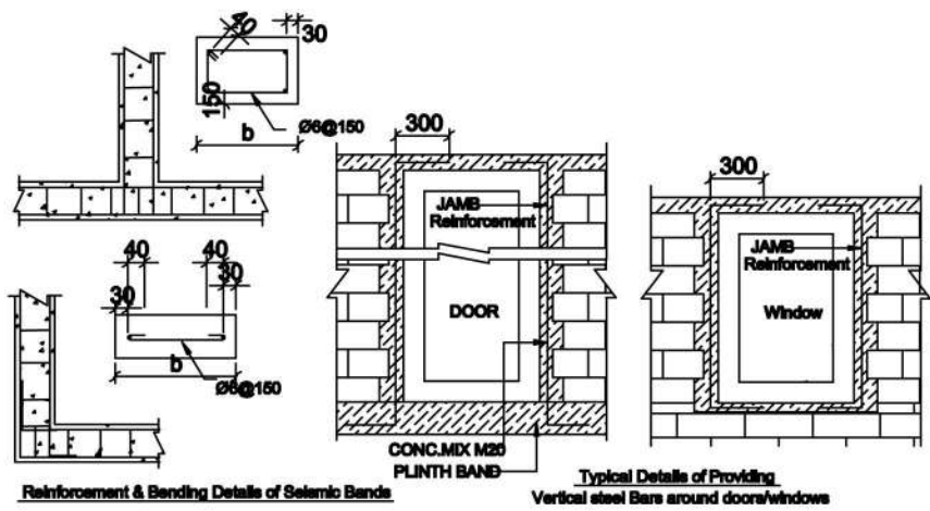
ESSEENTIAL INTERNAL ELEMENTS IN BUILDING
