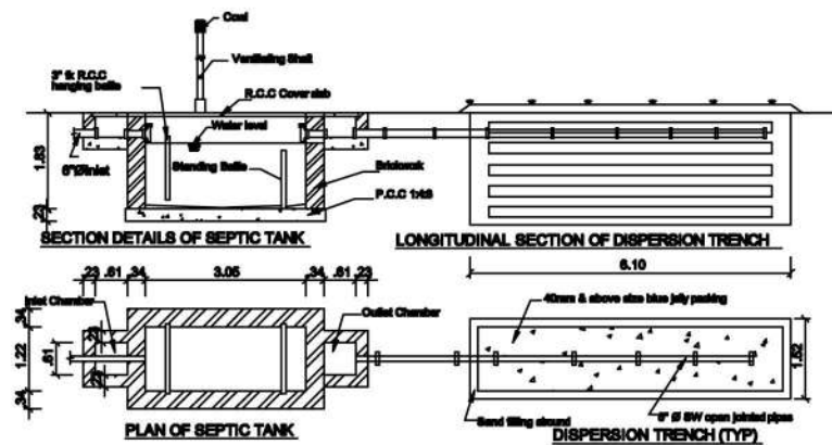
DETAILS OF SEPTIC TANK - 250 GALLONS
