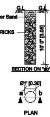
Rain Water Percolation Pit
