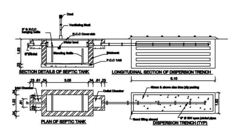
DETAILS OF SEPTIC TANK - 250 GALLONS
