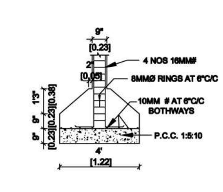
Column Foundation Details
