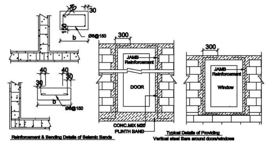
ESSENTIAL INTERNAL ELEMENTS IN BUILDING
