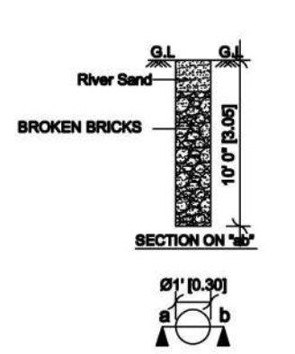
Rain Water Percolation Pit
