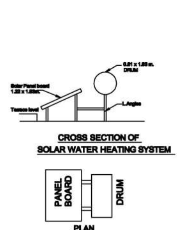
Solar Water Heater
