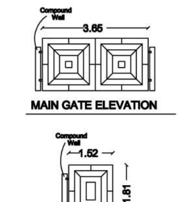
WICKET GATE ELEVATION
