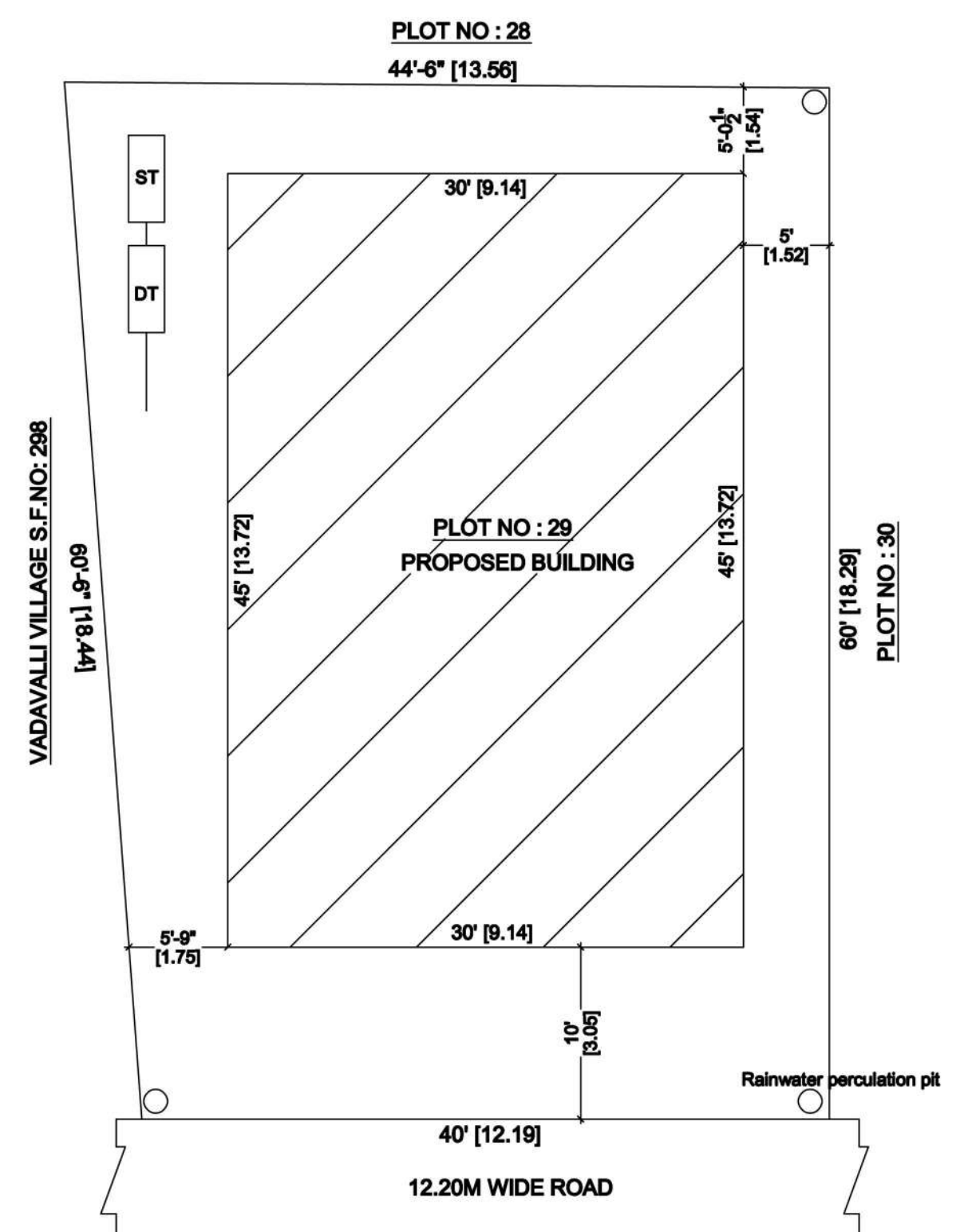
SITE PLAN
