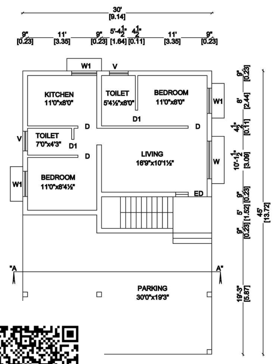
ND FLOOR PLAN
