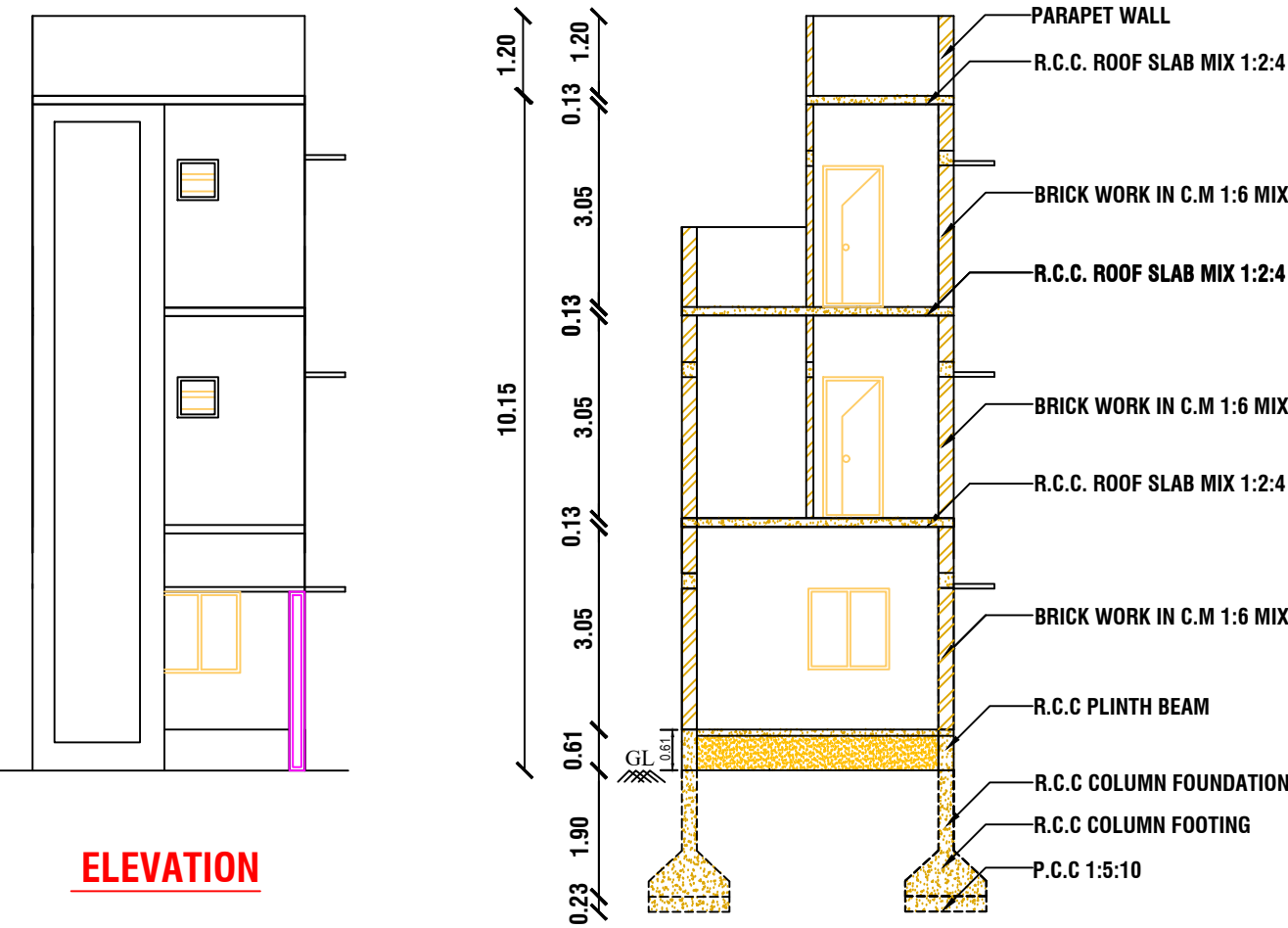
CROSS SECTION AT A-A
