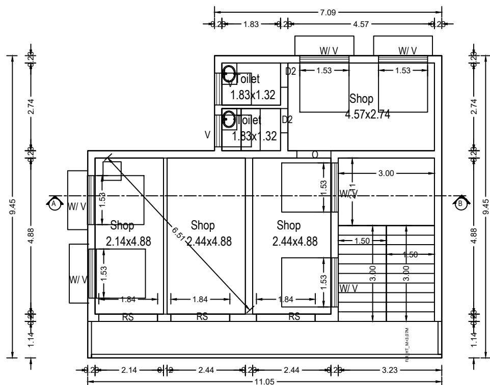
Pro First Floor Plan Scale 1:100
