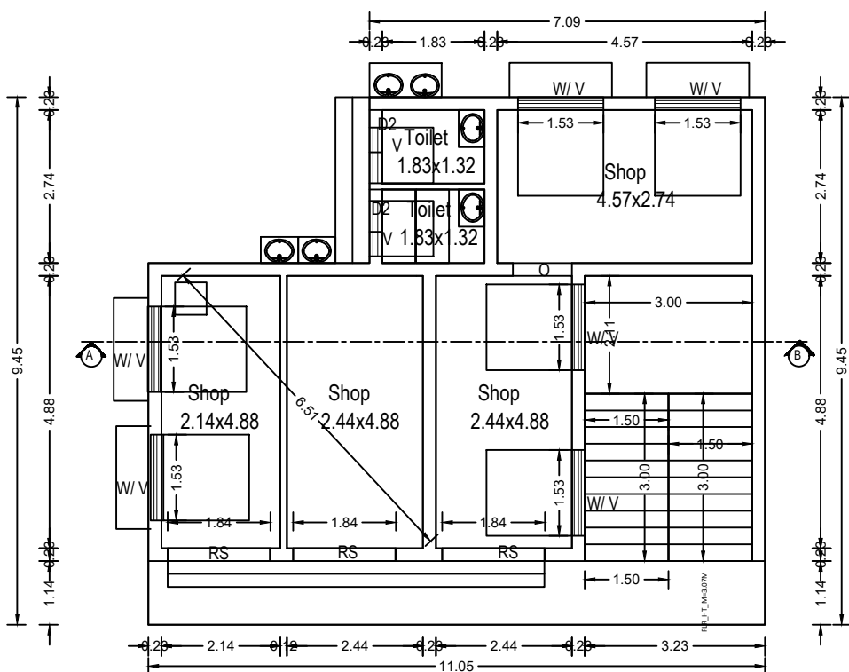
Exg Ground Floor Plan Scale 1:100
