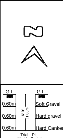
Trial - Pit (Not to Scale)
