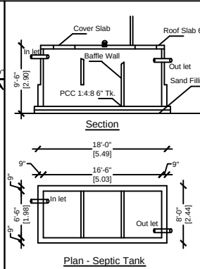
Plan - Septic Tank
