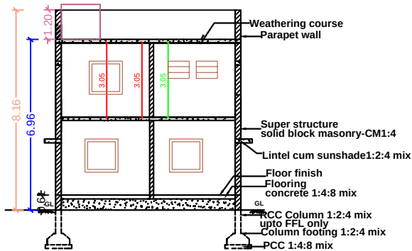
SECTION ELEVATION
