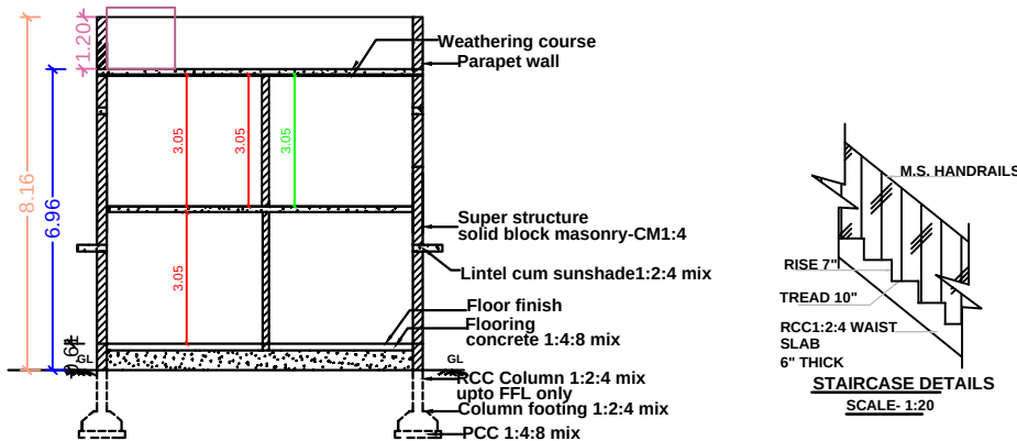
SECTION ELEVATION
