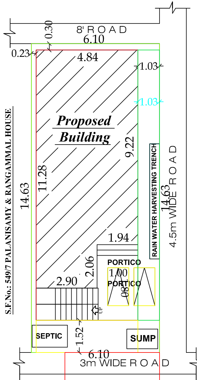
SITE PLAN
