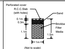
RAIN WATER HARVESTING RECHARGE TRENCH SECTION
