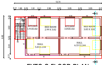
EXTG.G.FLOOR PLAN
