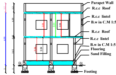
SECTION AB
