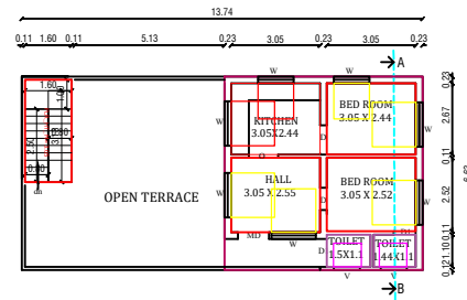
PRO.F.FLOOR PLAN
