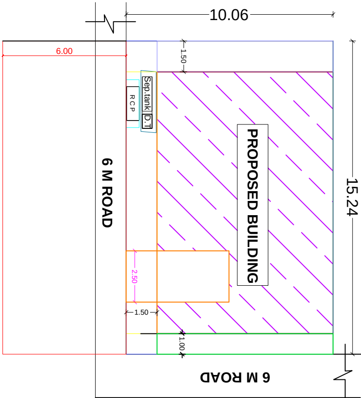
SITE PLAN
