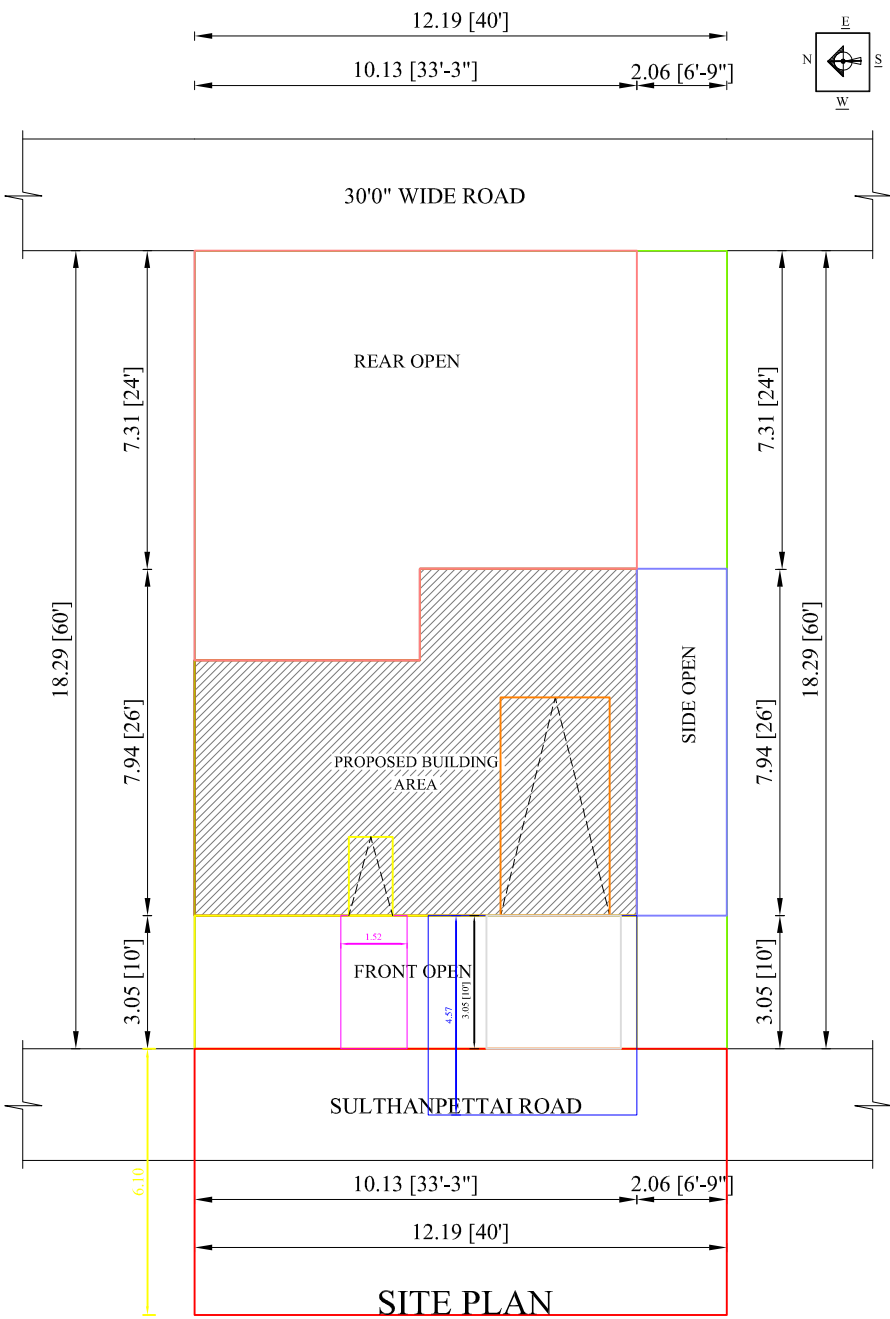
SITE PLAN
