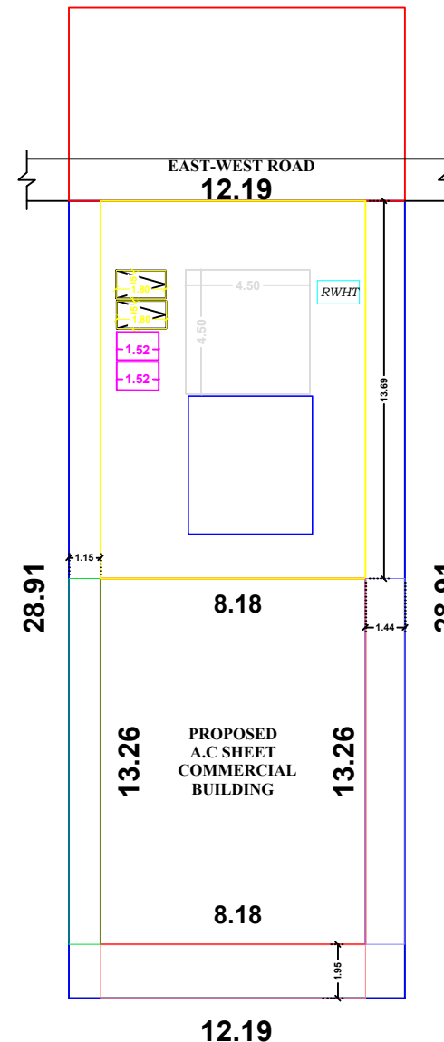
OWNER'S REMAINING LAND SITE PLAN
