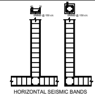
HORIZONTAL SEISMIC BANDS
