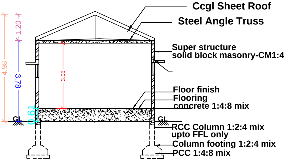
SECTION ELEVATION
