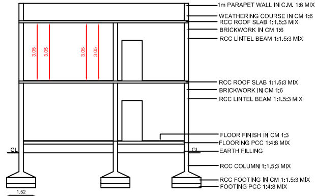
CROSS SECTION ON XY
