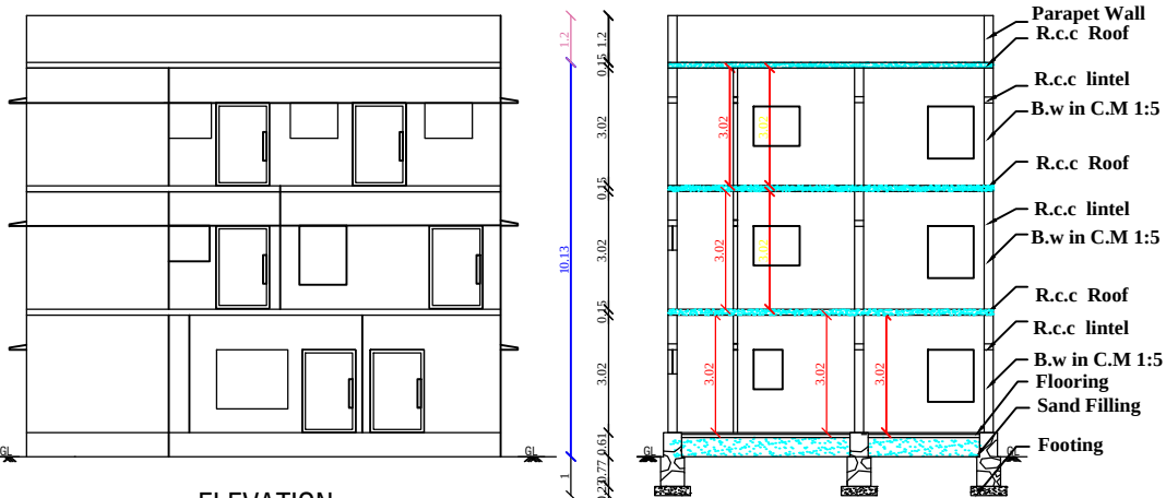
SECTION AB
