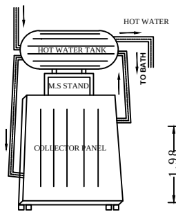
SOLAR WATER HEATER SYSTEM
