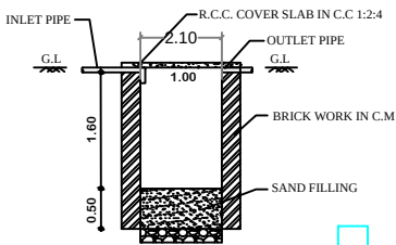
SECTIONAL DETAILS
