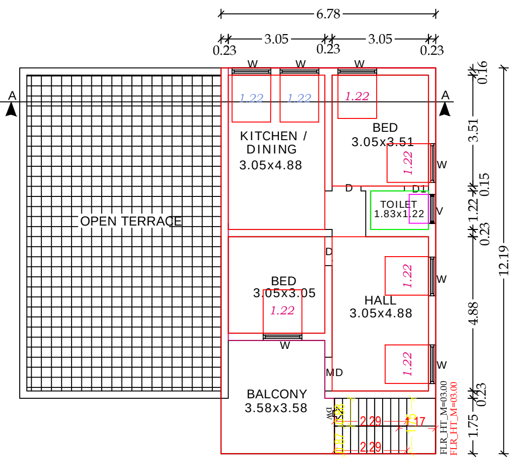
PRO. ADD. FIRST FLOOR PLAN
