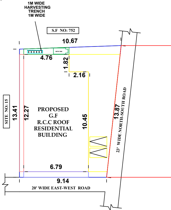
SITE PLAN
