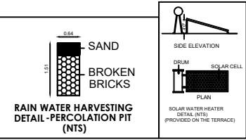
RAIN WATER HARVESTING DETAIL - PERCOLATION PIT (NTS)
