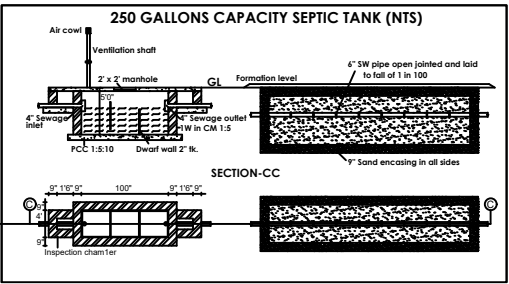
250 GALLONS CAPACITY SEPTIC TANK (NTS)
