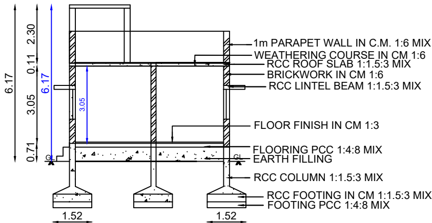
CROSS SECTION ON XY
