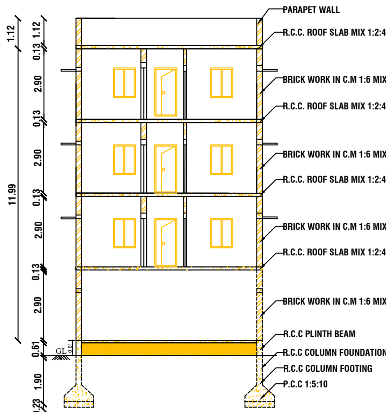
CROSS SECTION AT A-A
