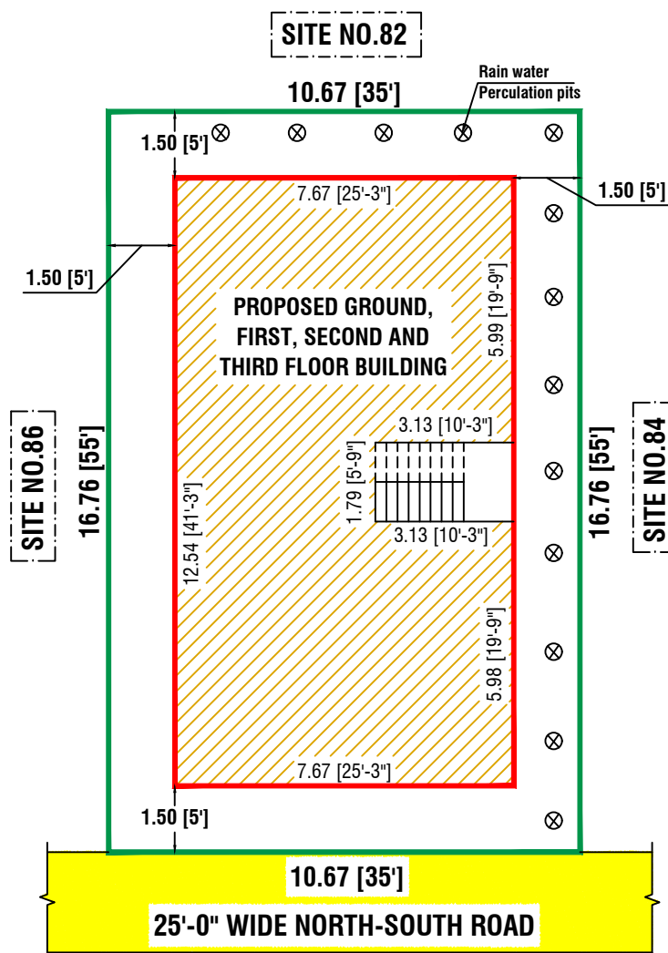
SITE PLAN
