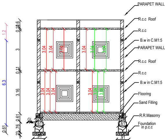
SECTION ,AB
