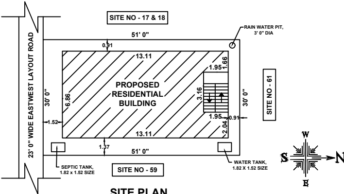
SITE PLAN
