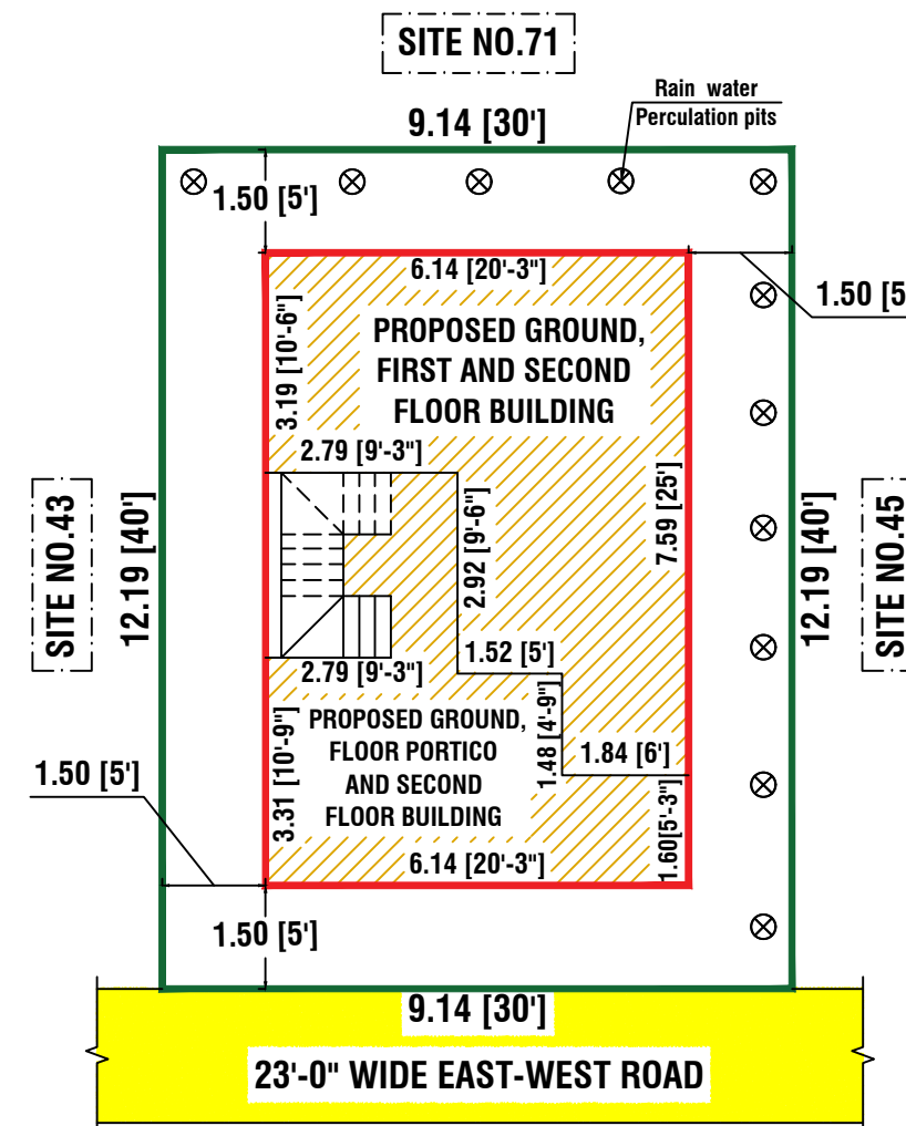
SITE PLAN
