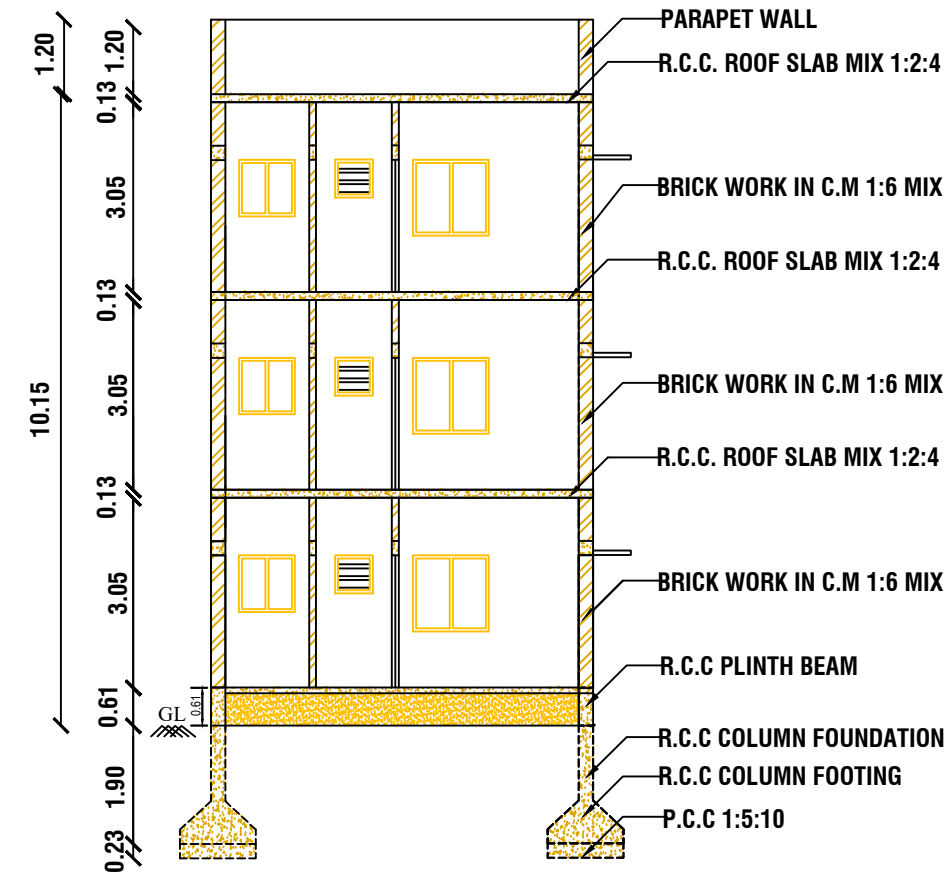
CROSS SECTION AT A-A
