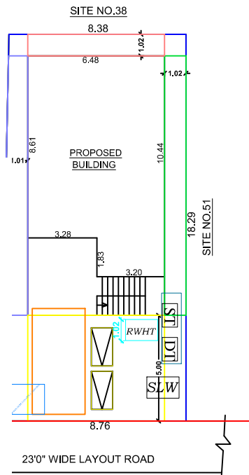
SITE PLAN
