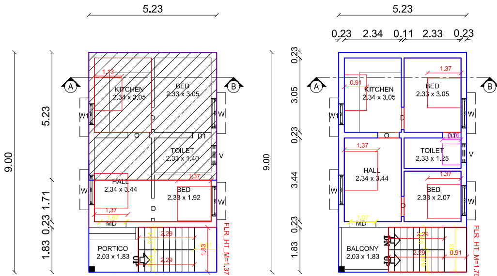
EXISTING & PRO.ADDL. GROUND FLOOR PLAN
