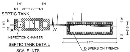
SEPTIC TANK DETAIL SCALE: NTS
