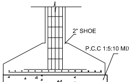
FOOTING DETAIL SCALE: NTS
