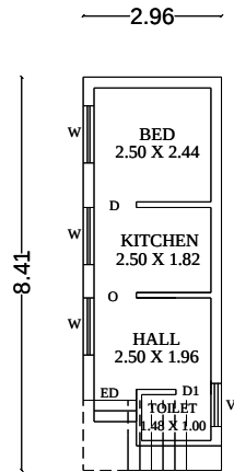
G.F. PLAN
