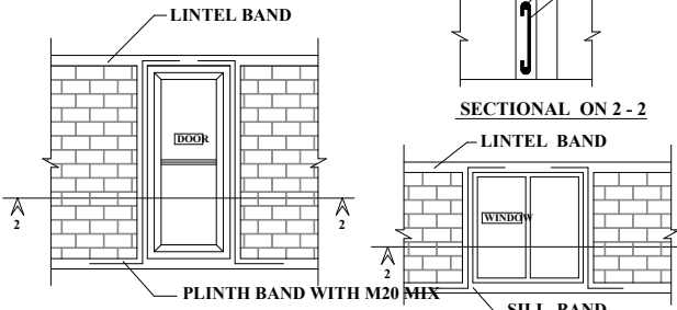
Figure - 2 : Reinforcement and Bending Details of Seismic Bands.
