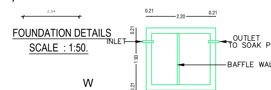
PLAN SEPTIC. TANK
