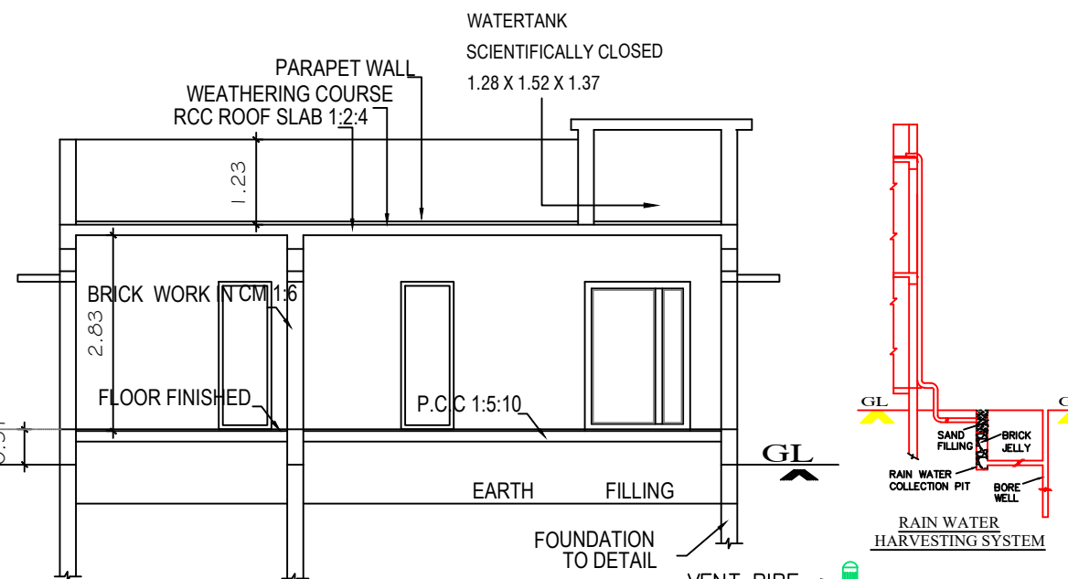
SECTION "A-B"
