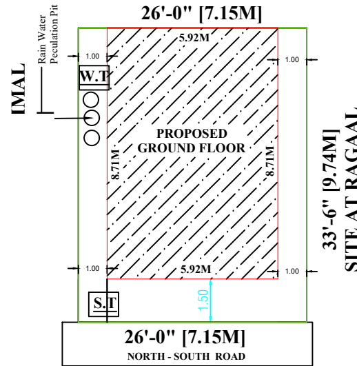
SITE PLAN
