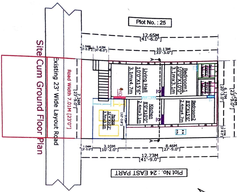
Site cum Ground Floor Plan
