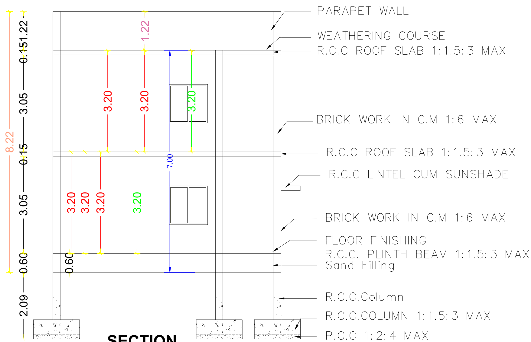
SECTION
