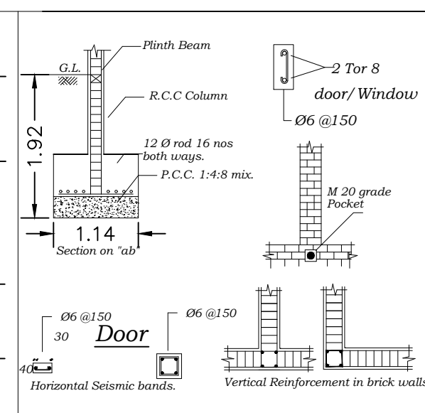
Horizontal Seismic bands
