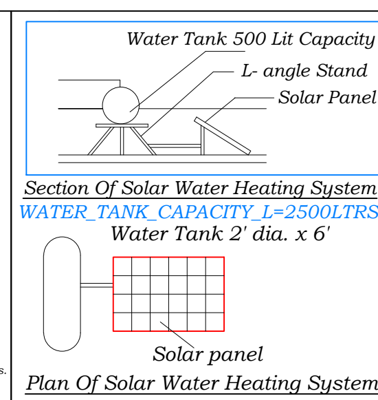
Plan Of Solar Water Heating System
