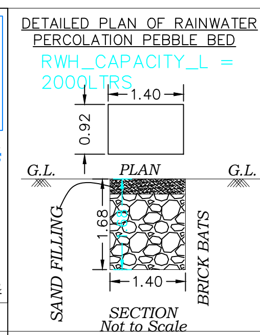
SECTION Not to Scale
