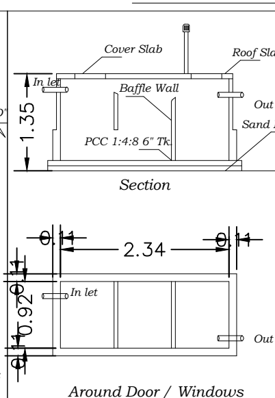
Around Door / Windows
