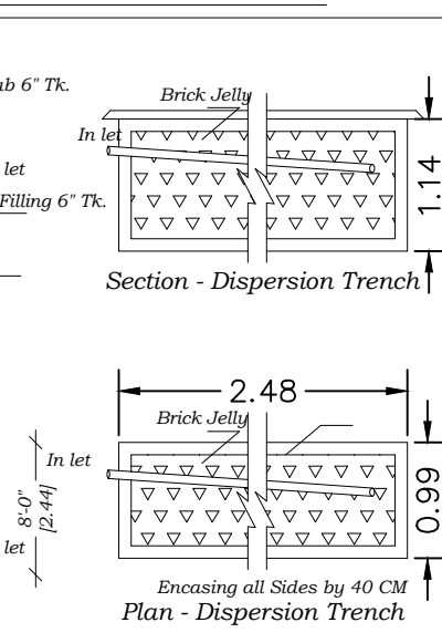
Plan - Dispersion Trench
