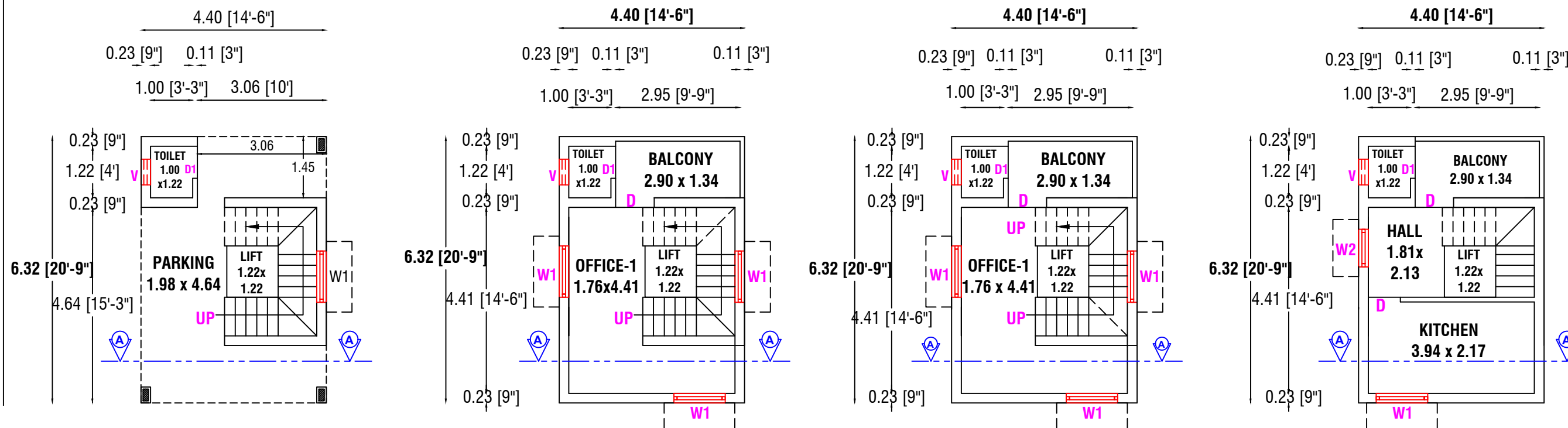
REVISED FIRST FLOOR PLAN
