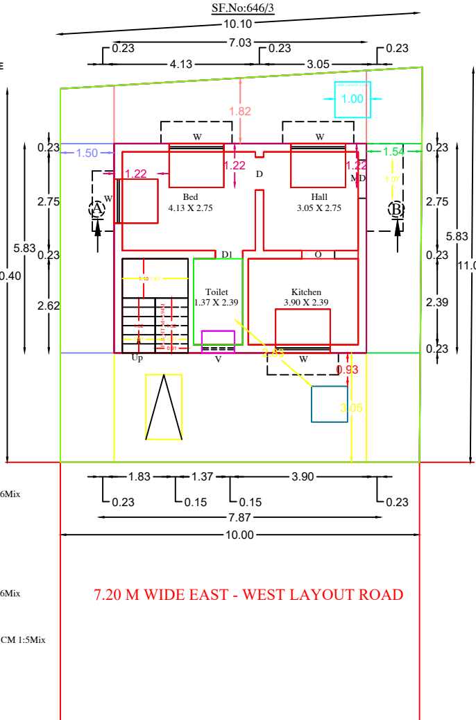
SITE PLAN & PROPOSED GROUND FLOOR PLAN
