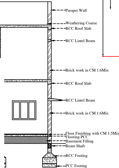
SECTION "AB"
