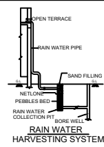
RAIN WATER HARVESTING SYSTEM
