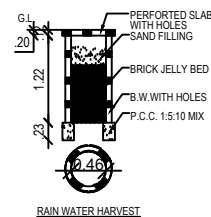
RAIN WATER HARVEST
