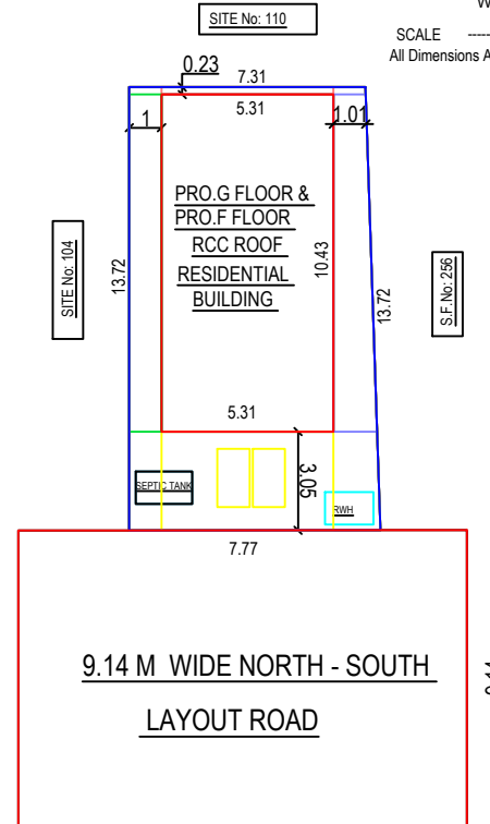
SITE PLAN
