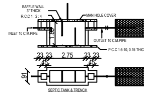
SEPTIC TANK & TRENCH
