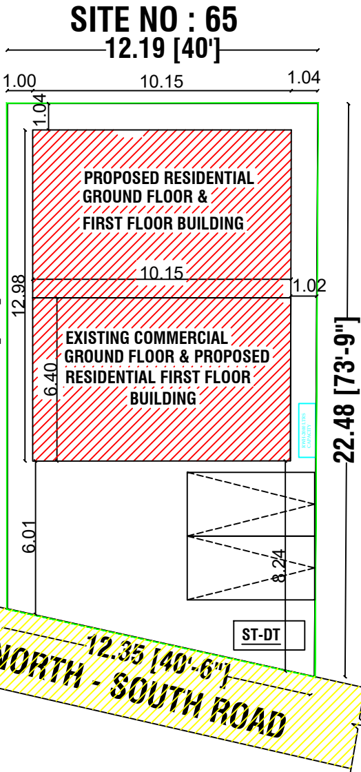
SITE PLAN
