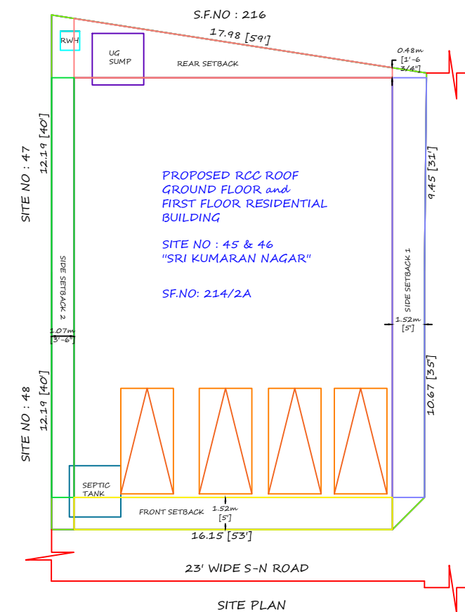
SITE PLAN
