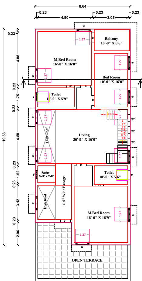
PRO.FIRST FLOOR PLAN
