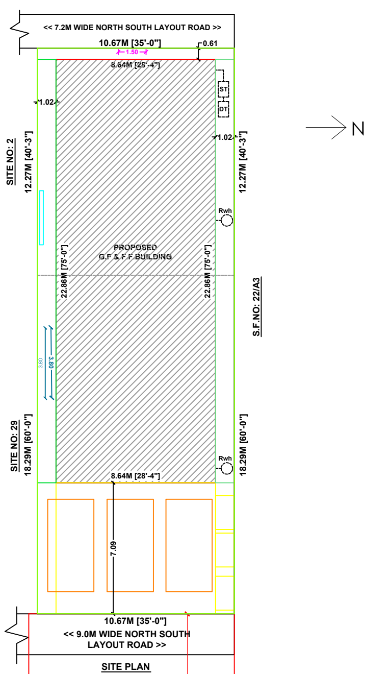
SITE PLAN
