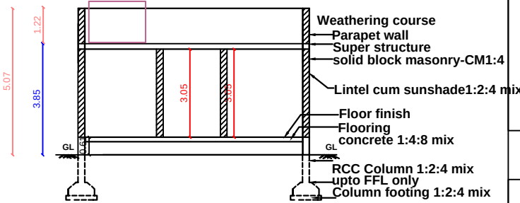
SECTION ELEVATION
