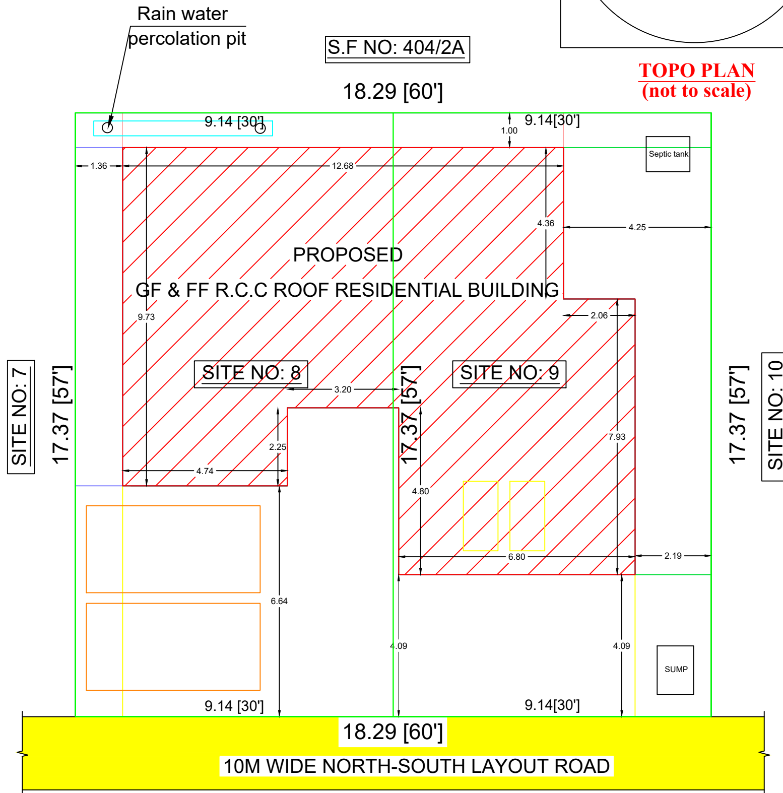
SITE PLAN
