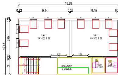
PROPOSED ADDITIONAL FIRST FLOOR BUILDING
