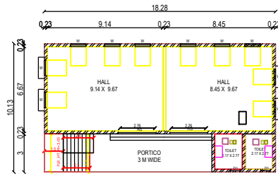
EXISTING BUILDING D.NO. 3/319/A
