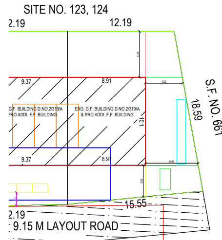
PROPOSED ADDITIONAL FIRST FLOOR BUILDING
