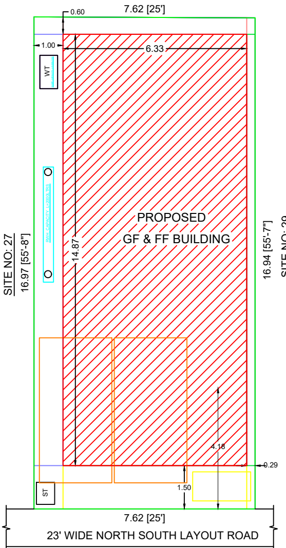
SITE PLAN
