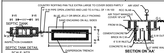
SEPTIC TANK DETAIL SCALE: NTS
