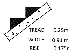
STAIRCASE DETAIL:
