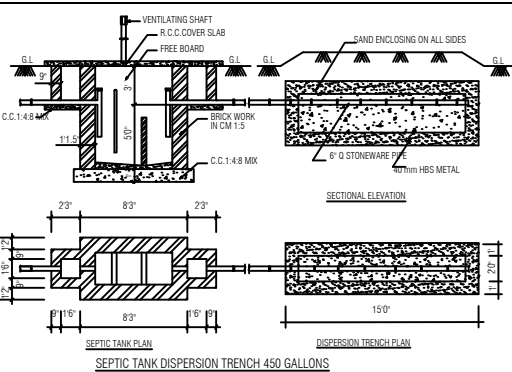
SEPTIC TANK SECTION
