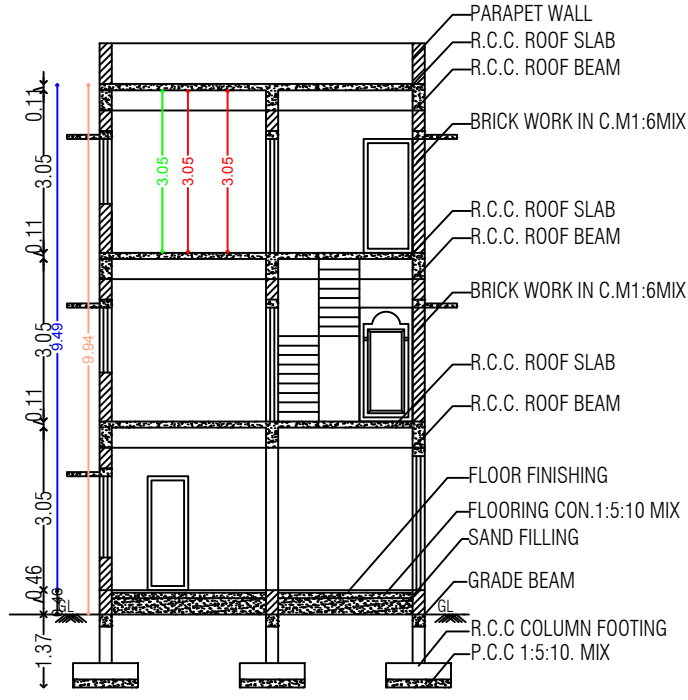
SECTION ON "AA" (Scale :- 1"Eq8'0")
