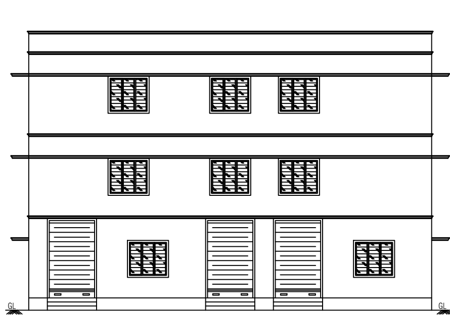
FRONT ELEVATION (Scale :- 1"Eq8'0")
