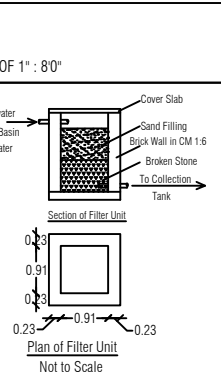
COLLECTION UNIT SECTION
