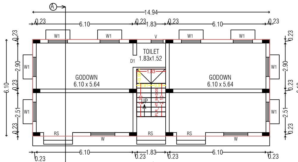
GROUND FLOOR PLAN (Scale :- 1"Eq8'0")
