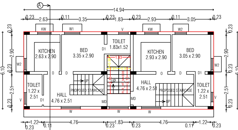
FIRST FLOOR PLAN (Scale :- 1"Eq8'0")
