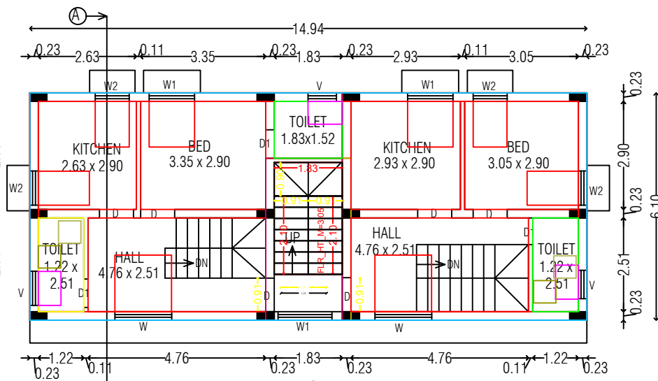
SECOND FLOOR PLAN (Scale :- 1"Eq8'0")
