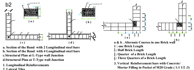
3. Vertical Reinforcement at corners
